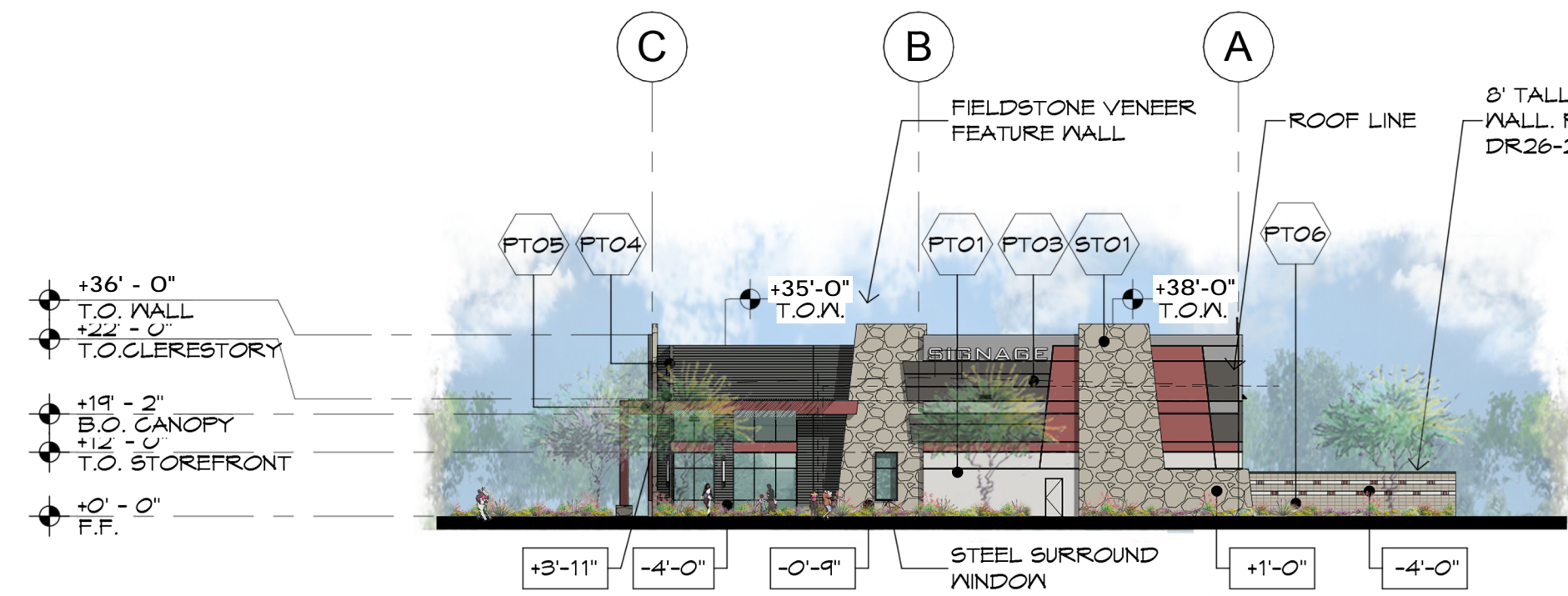
2 BLDG I - EAST SCALE: 1" = 30'-0"
