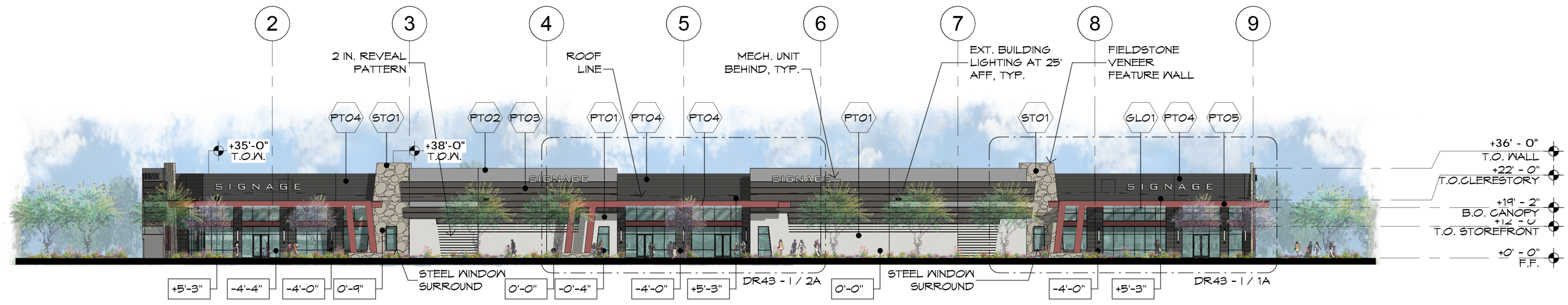
1 BLDG I - SOUTH SCALE: 1" = 30'-0"
