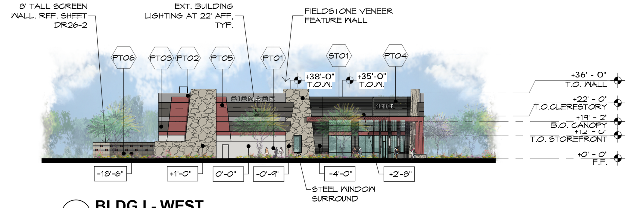
3 BLDG I - WEST SCALE: 1" = 30'-0"
